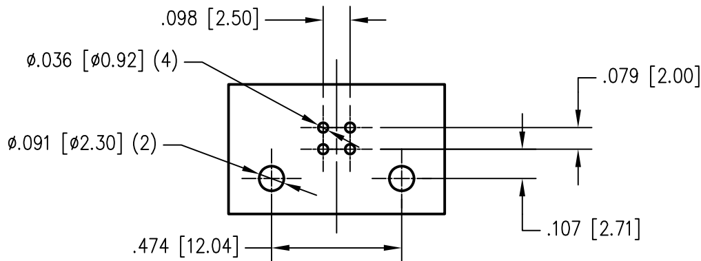
RECOMMENDED P.C.B. HOLE LAYOUT TOP VIEW (TOLERANCE ± .002 [0.05])
