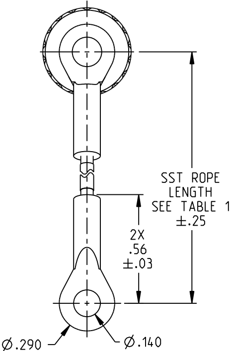
RFIX457XX-12 THRU RFIX457XX-17 SST ROPE & MTG LUG
