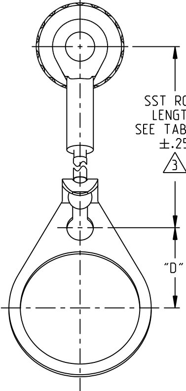
RFIX457XX-12-D2 THRU RFIX457XX-17-DD8 SST ROPE w/BULKHEAD MTG LUG
