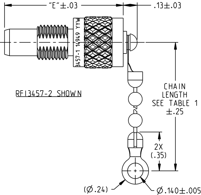
RFIX457XX-2 THRU RFIX457XX-11 BEAD CHAIN & END RING
