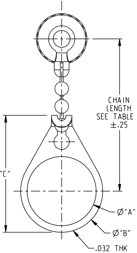
RFIX457XX-2-D2 THRU RFIX457XX-11-DD8 BEAD CHAIN w/BULKHEAD MTG LUG
